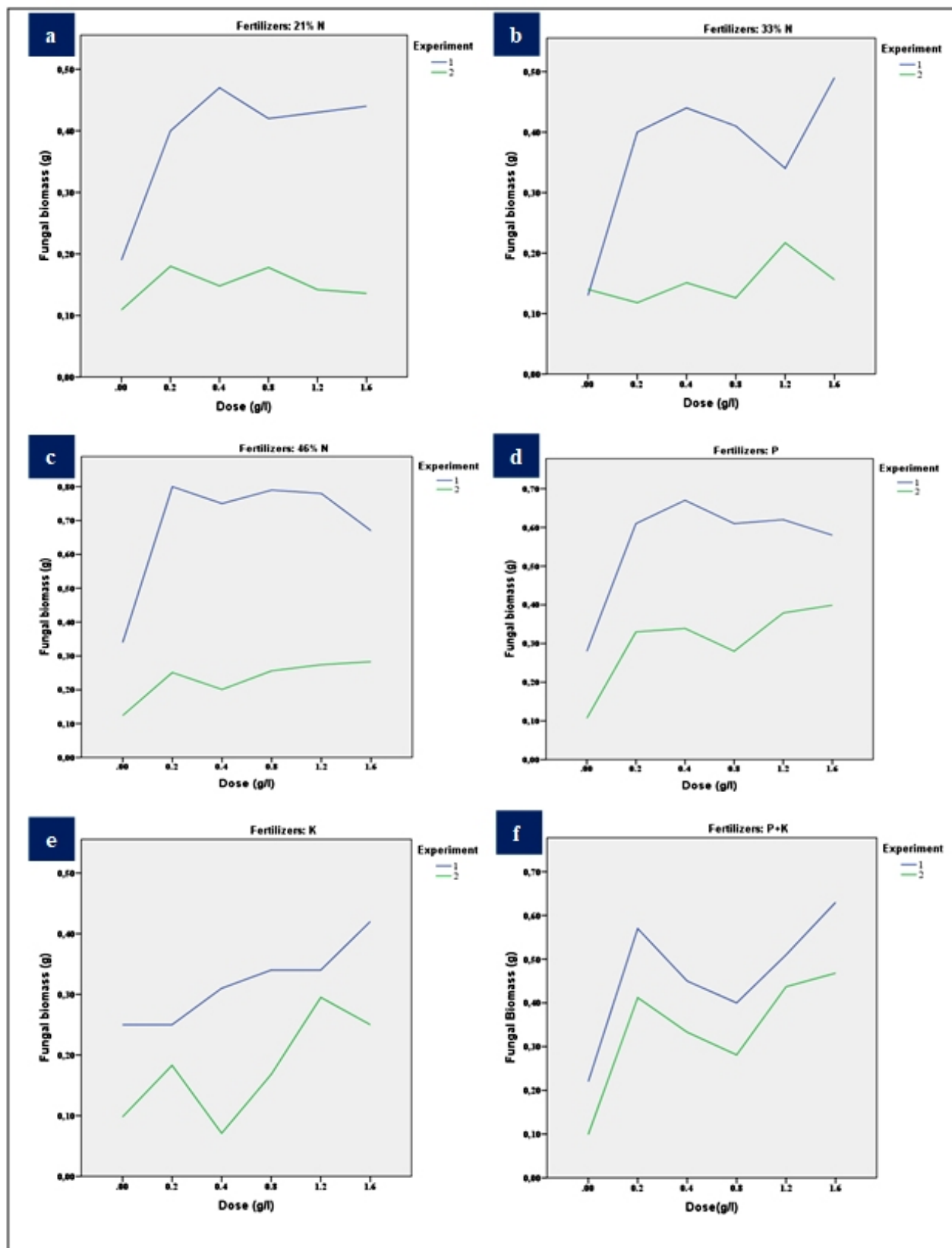
Figure 1. Effect of fertilizer's type and rates added to growth media on Fusarium culmorum fungal biomass production under two experimental conditions (experiment 1 : 20–25 °C; experiment 2: 15–20 °C). Note: 21% N: Ammonium sulfate (a); 33% N: Ammonium nitrate (b); 46% N: Urea (c); P: Phosphorus (d) and K: Potassium sulfate (e); P+K (f).
