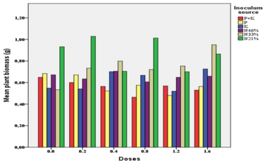
Figure 4. Differential effect of inoculum sources (fungus reared on media containing) fertilizers) and rates within fertilizers on dry weight biomass of inoculated plants. Note: The inoculum source represent the fungus that wa was reared on the fertilizers used, and none of the fertilizers was added to the inoculated plants.
